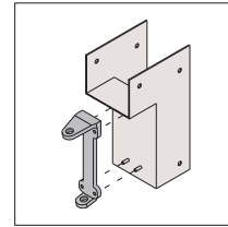
Extension 'L' bracket
